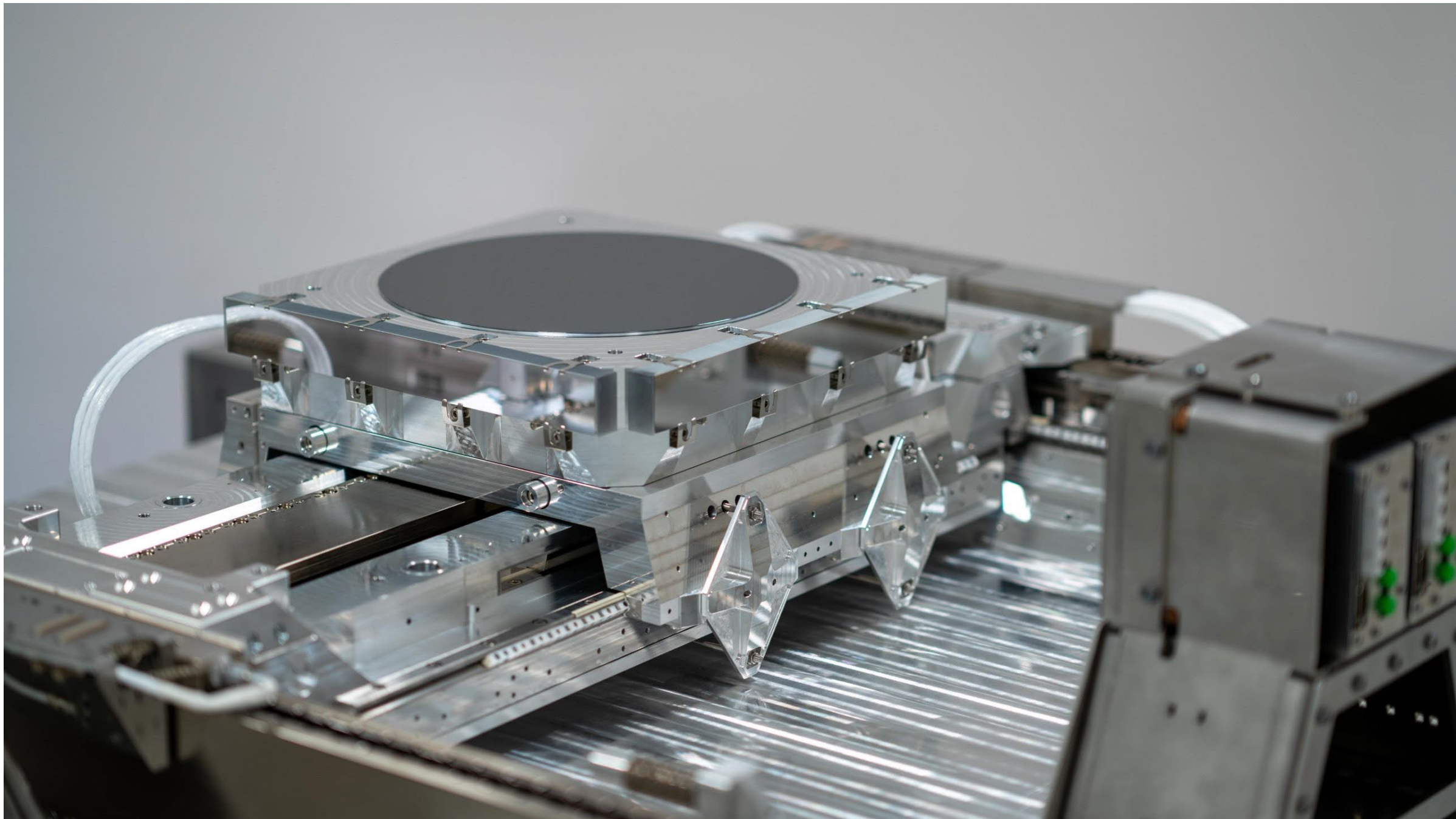
Off the shelf motion stage for wafer inspection, powered by Apogee and Kepler drives
